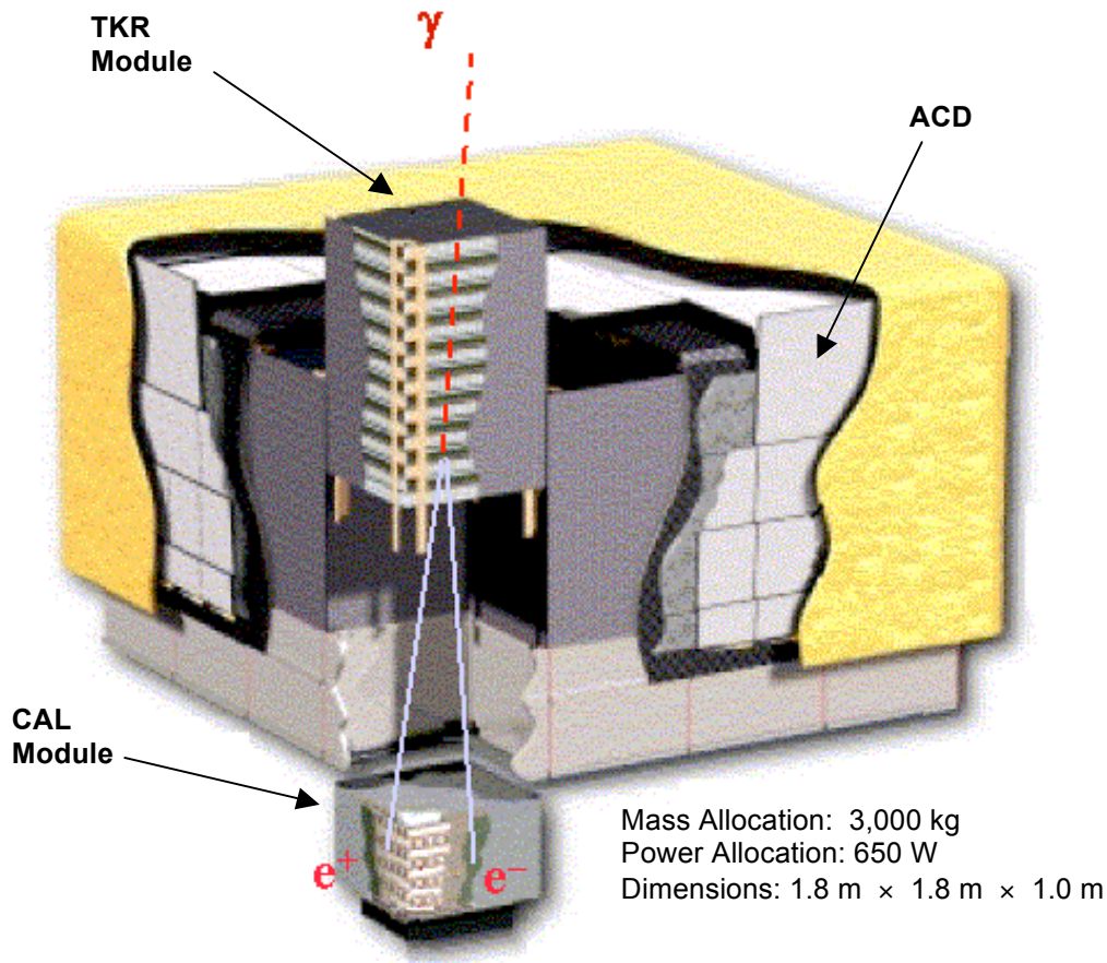
Figure 3-1: LAT Instrument Schematic
