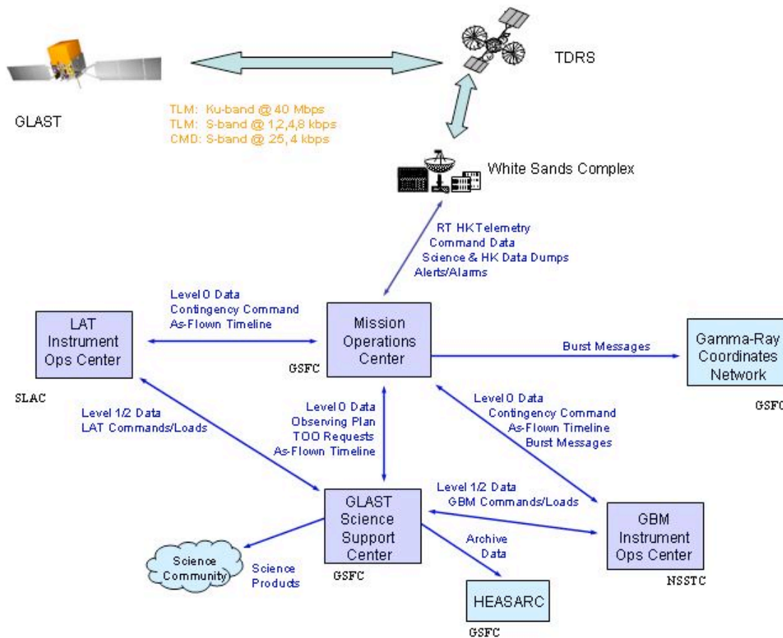
Figure 4-1: GLAST Ground Operations Overview. Only the elements involved in the data management during normal operations are shown.
