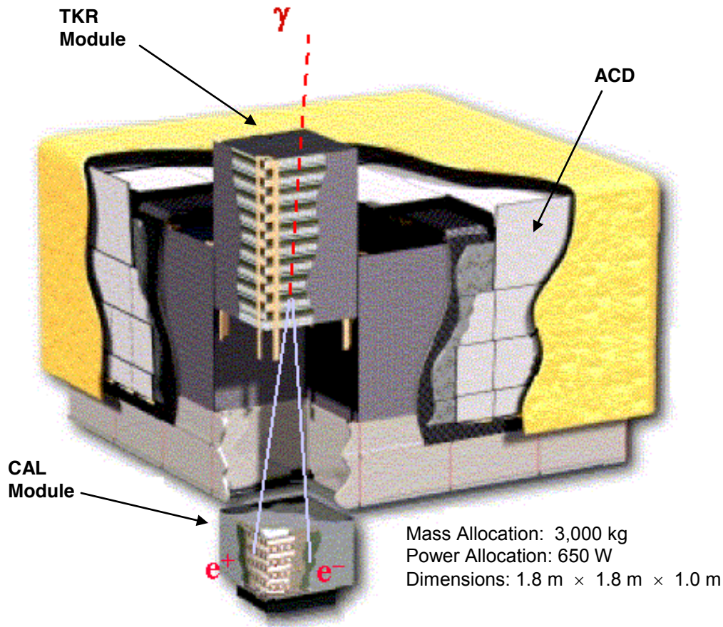
Figure 3-1: LAT Instrument Schematic
