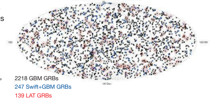
Fermi GRBs as of November 26, 2017
