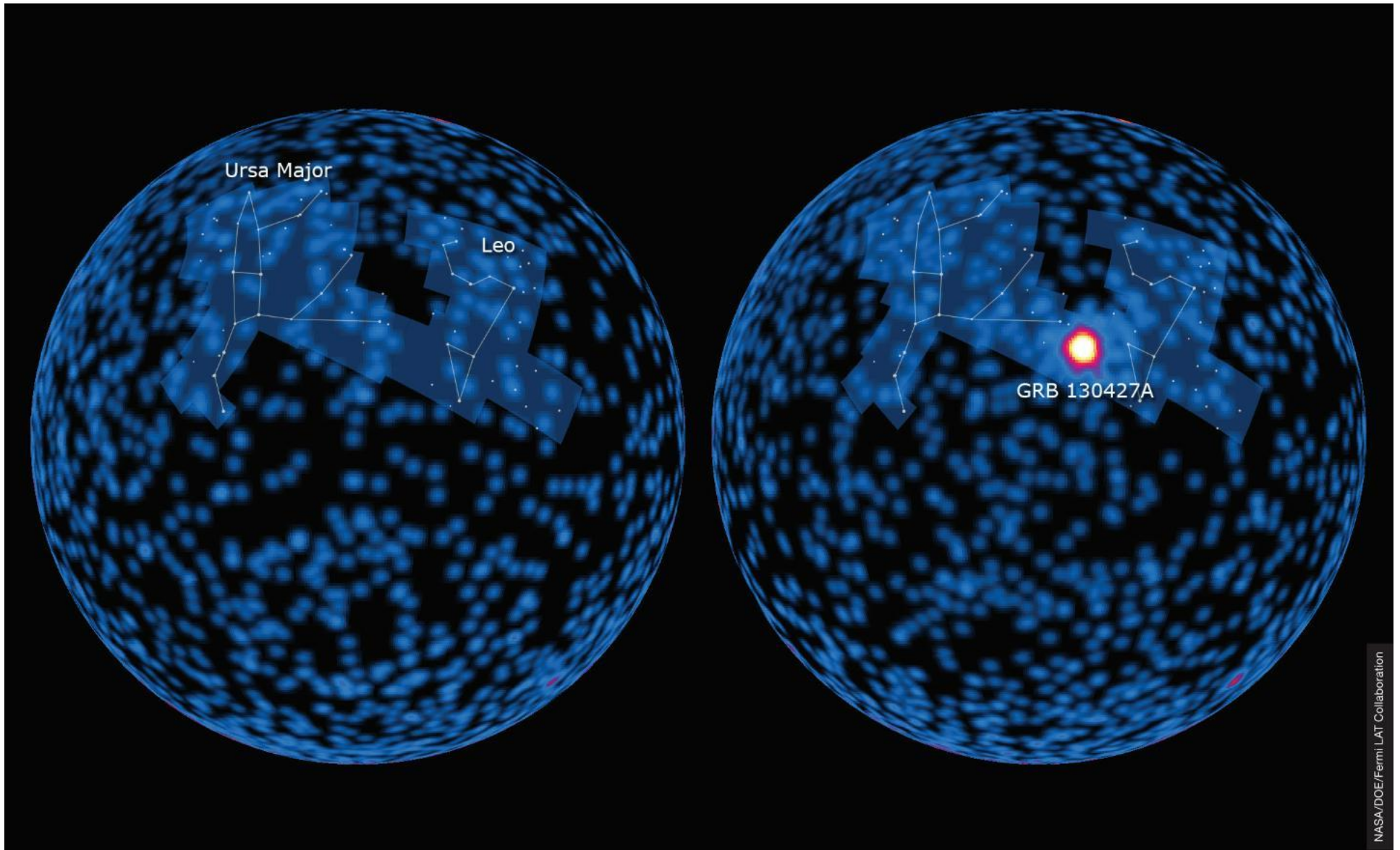
Before and after Fermi LAT views of GRB 130427A, centered on the north galactic pole. For more information visit http://fermi.gsfc.nasa.gov/
