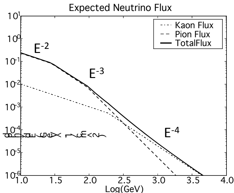
Above: Model flux for 'choked' GRB event.
