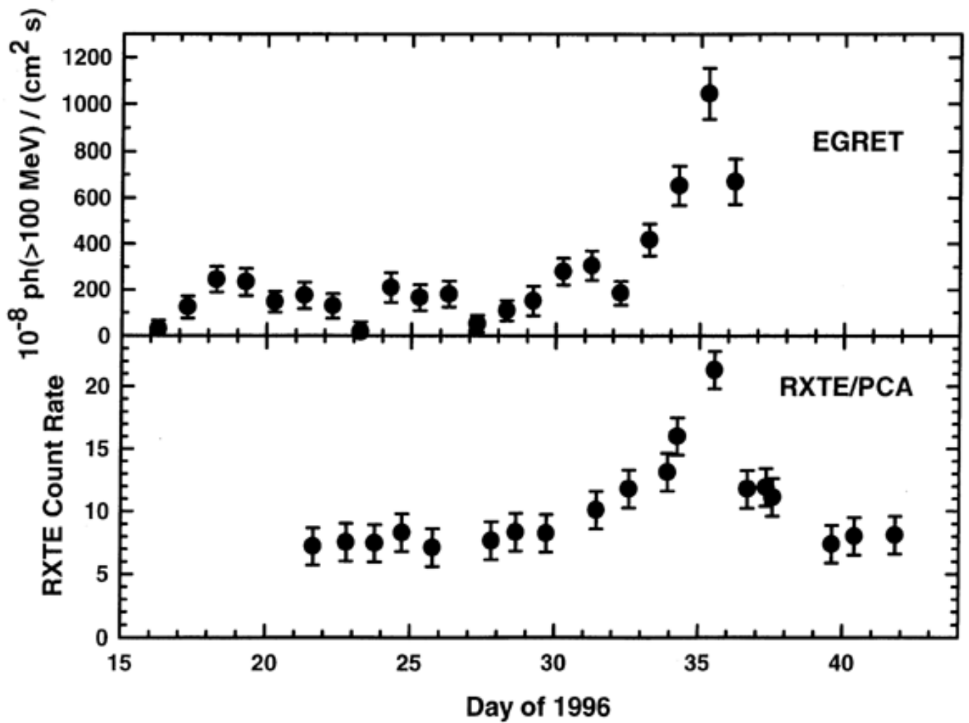
Figure 3 - Light curves for \gamma -rays and X-rays in 1996
