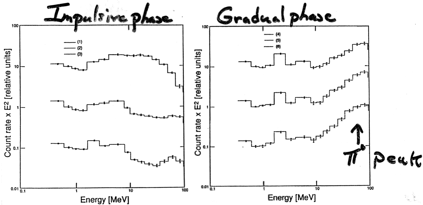
Figure 5. The \gamma -ray spectrum (weighted by E^2 ) from the (a, left) impulsive and transitional and (b, right) the gradual phase periods of the 24 May 1990 flare.
