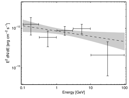
3FGL J0758.9+2705 - SDSS J075846.99+270515.5
