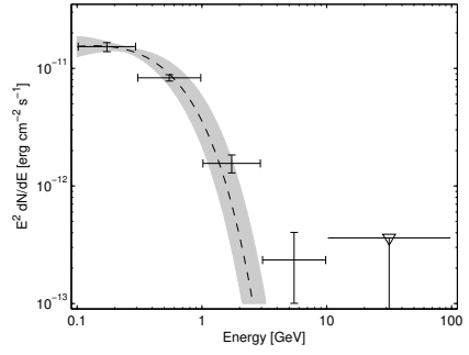
3FGL J0659.5+1414 – PSR J0659+1414
