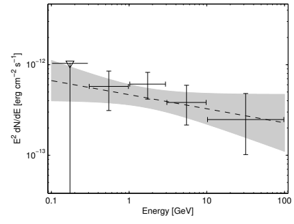
3FGL J0758.7+3747 - NGC 2484
